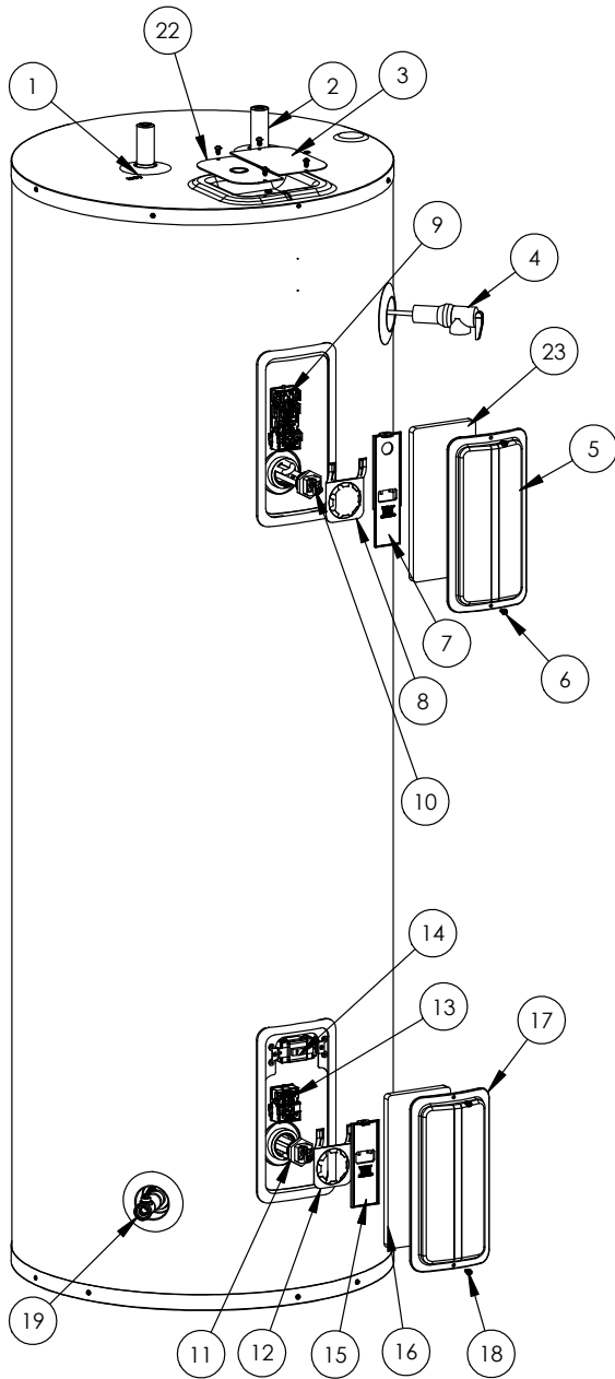
Figure 8 - Replacement Parts
